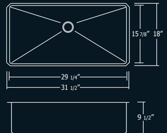
31 1/2" x 18" x 9 1/2" Minimum Cabinet Size: 33" Single Bowl, 16 Gauge
