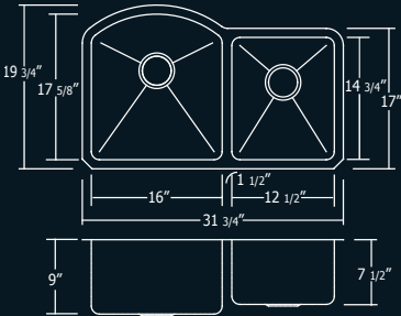
31 3/4" x 19 3/4" x 9" Minimum Cabinet Size: 33" Large & Small Bowl, 16 Gauge
