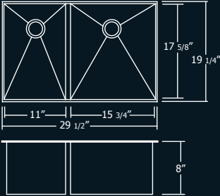
29 1/2" x 19 1/4" x 8" Minimum Cabinet Size: 33" Large & Small Bowl, 18 Gauge
