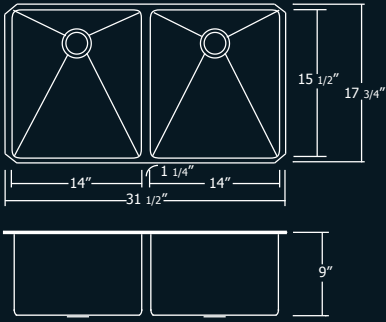
31 1/2" x 17 3/4" x 9" Minimum Cabinet Size: 33" Double Bowl, 16 Gauge
