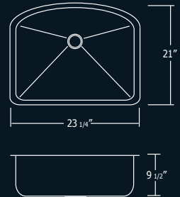
23 1/4" x 21" x 9 1/2" Minimum Cabinet Size: 27" Single Bowl, 16 Gauge
