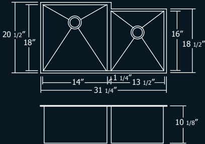
31 1/4" x 20 1/2" x 10 1/8" Minimum Cabinet Size: 33" Large & Small Bowl, 18 Gauge
