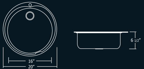
20" x 20" x 6 1/2" Minimum Cabinet Size: 21" Round Bar Sink, 22 Gauge
