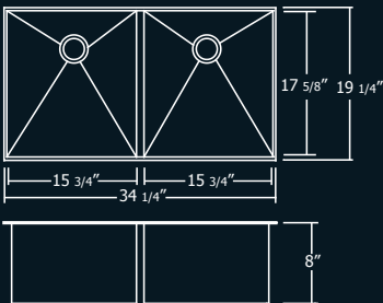
34 1/4" x 19 1/4" x 8" Minimum Cabinet Size: 36" Double Bowl, 18 Gauge
