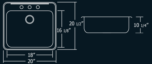
20" x 20 1/2" x 10 1/4" Minimum Cabinet Size: 21" Deep Laundry Sink, 19 Gauge
