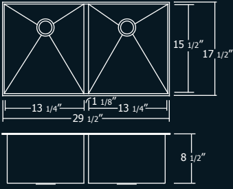
29 1/2" x 17 1/2" x 8 1/2" Minimum Cabinet Size: 33" Double Bowl, 18 Gauge
