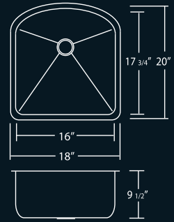
18" x 20" x 9 1/2" Minimum Cabinet Size: 21" Single Bowl, 16 Gauge
