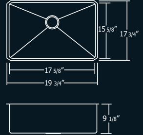
19 3/4" x 17 3/4" x 9 1/8" Minimum Cabinet Size: 24" Single Bowl, 16 Gauge
