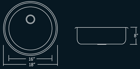
18" x 18" x 8" Minimum Cabinet Size: 21" Round Bar Sink, 20 Gauge
