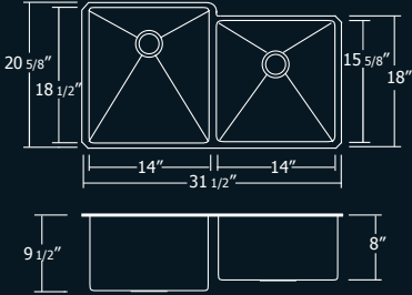
31 1/2" x 20 5/8" x 9 1/2" Minimum Cabinet Size: 33" Large & Small Bowl, 16 Gauge
