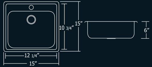
15" x 15" x 6" Minimum Cabinet Size: 18" Square Bar Sink, 24 Gauge
