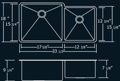
33 1/2" x 18" x 9 1/4" Minimum Cabinet Size: 36" Large & Small Bowl, 16 Gauge
