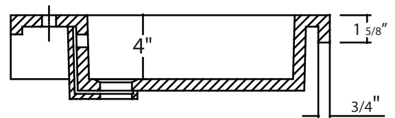
A-A Cut View
